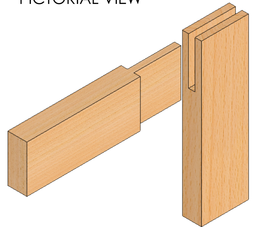
EXPLODED VIEW
